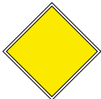
paratrooper landing
